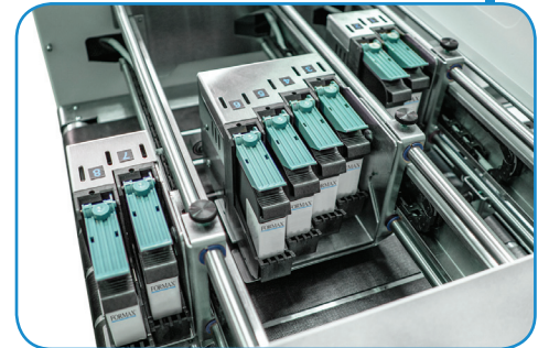
Three independent print heads: 2-pen + 4-pen + 2-pen stitched design
